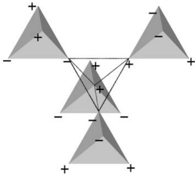
Figure 2. In the ground state (found originally by enumeration of clusters of 16 sites), each tetrahedron satisfies the Ice rules i.e. two spins point in and two point out, and yet the crystal has true long ranged order. The nature of the order is visualized in the top view here (from R. Siddharthan et. al, Phys. Rev. B 63, 184412 (2001)).
