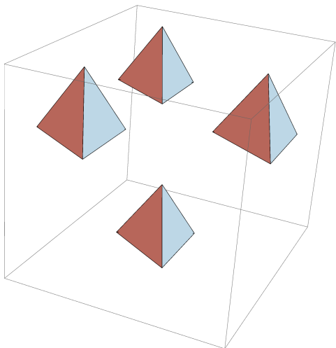
Figure 1. The pyrochlore lattice can be built up with a basis of four tetrahedra as seen in the side view here. We populate this lattice with Ising spins on the corners, pointing either in or out of each tetrahedron along the local axis pointing to the center.
